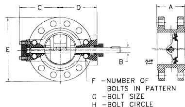
DOUBLE FLANGE
