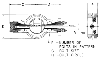
WAFER
